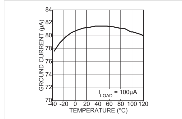
FIGURE 2-5: Ground Pin Current.
