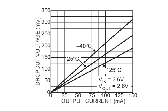
FIGURE 2-10: Dropout Voltage.
