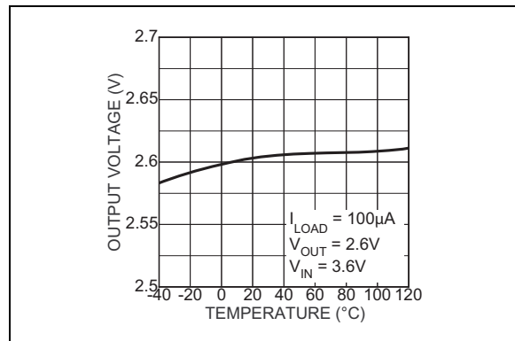
FIGURE 2-12: Output Voltage vs. Temperature.
