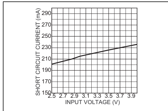
FIGURE 2-11: Short Circuit Current.
