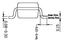
END VIEW
